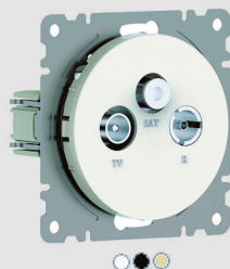
TV-RF-SAT Antenna Socket End Piece in Box / Package - 5 /100
