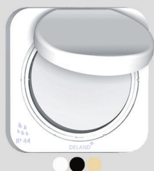
One Way Switch Illuminated With Lid 10A , 250 V~ Piece in Box / Package - 5 /100
